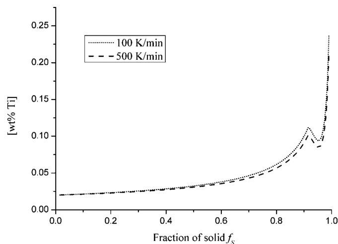
Fig. 3. Titanium segregation during solidification of steel 1 at the cooling rate of 100 K/min and 500 K/min
