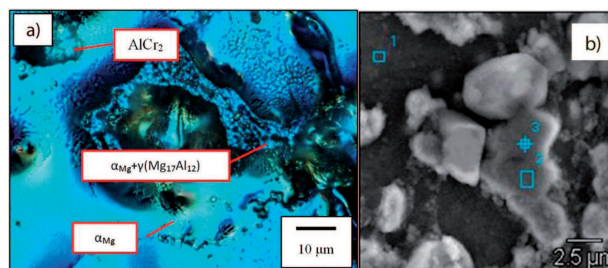
Fig. 3. Microstructure of AM60 +0.1% Cr alloy solidifying in a ceramic mold observed by means of optic microscope (a) and scanning microscope (b)
