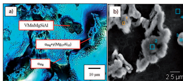
Fig. 2. Microstructure of AM60 +0.1% V alloy solidifying in a ceramic mold observed by means of optic microscope (a) and scanning microscope (b)
