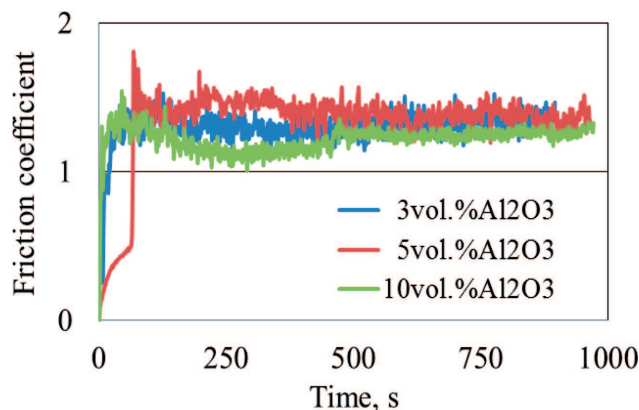
Fig. 5. The friction coefficient of copper-alumina composites
