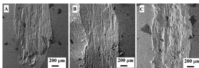
Fig. 6. SEM images of friction traces of \text{Cu-Al}_2\text{O}_3 composites after 15 min: a) 3 vol.% \text{Al}_2\text{O}_3 , b) 5 vol.% \text{Al}_2\text{O}_3 , c) 10 vol.% \text{Al}_2\text{O}_3
