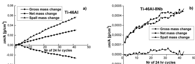
Fig. 5. Cyclic oxidation kinetics of a) Ti-46Al and b) Ti-46Al-8Nb at 1073 K in laboratory air for 42 cycles (1 cycle, 24 hrs)
