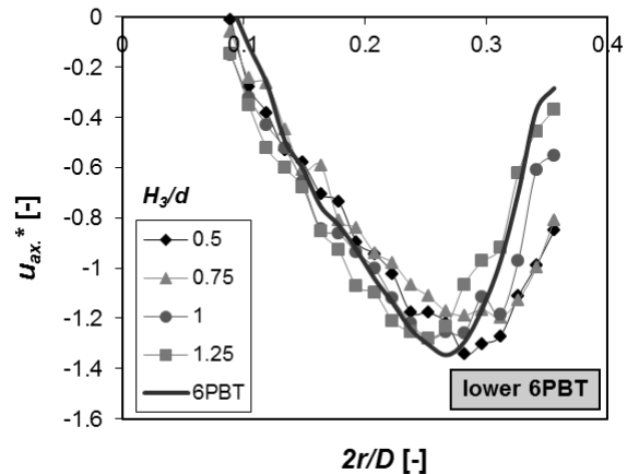
Fig. 5. Radial profile of the dimensionless axial component of the mean velocity in a liquid leaving the rotor region of upper three-blade and lower six-blade impeller constituted multi-stage impeller for various distance between impellers (thick solid line 6PBT – independently operating pitched six-blade impeller)
