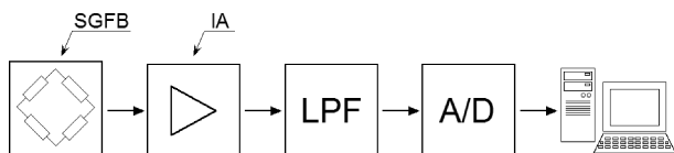
Fig. 4. Block diagram of the signal processing path for each of the six strain gauge transducers mounted in the posturographic platform, where: SGFB – Full Bridge Strain Gauge, IA – Instrumentation Amplifier, LPF – Low-Pass Filter, A/D – Analog to Digital Converter
