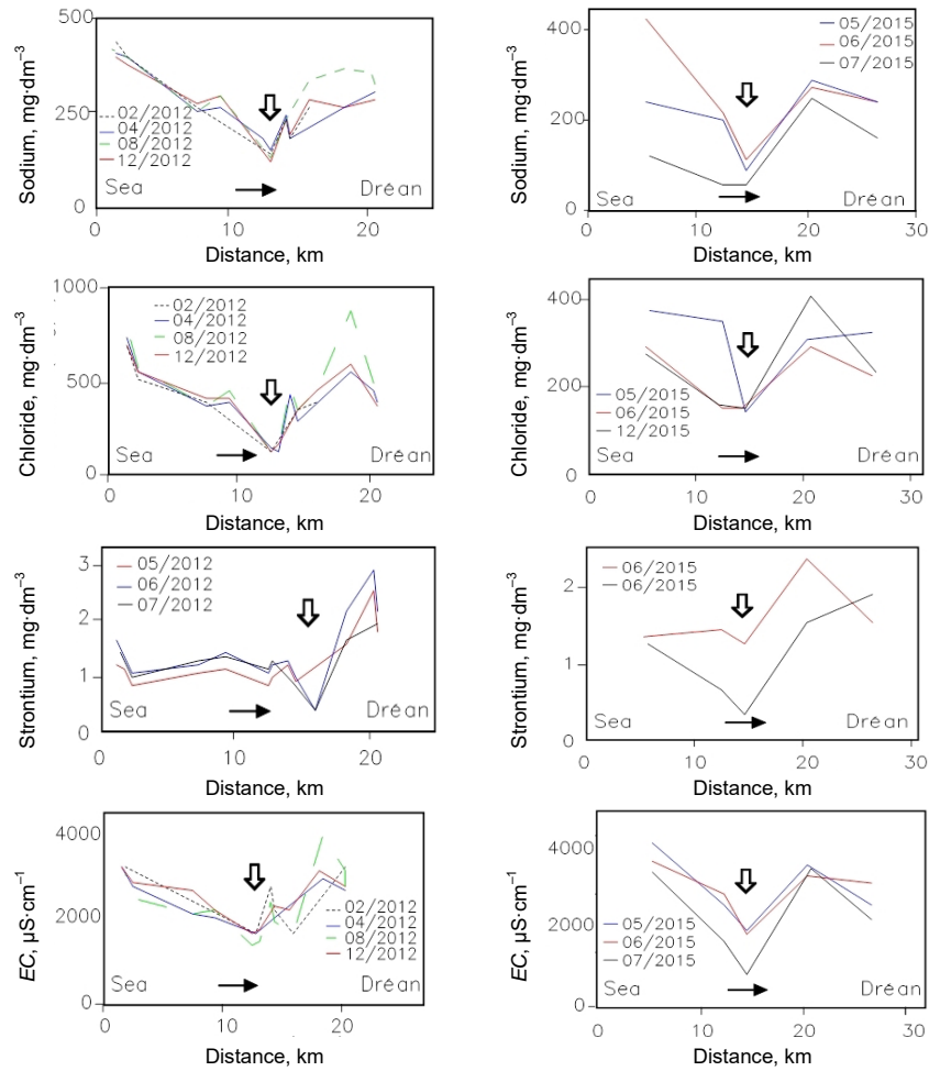
Fig. 5. Graphs for chlorides, sodium, strontium and electric conductivity (EC) from the sea to Dréan; source: own study
