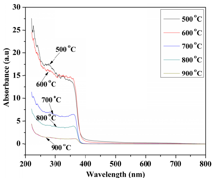
Fig. 7. UV-vis absorption spectra of the ZnO-SiO 2 nanocomposite calcined at various calcination temperatures
