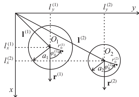
Fig. 2. Locations of the membranes on the horizontal baffle of the three-wall corner region: vectors describing the locations of sources' central points \mathbf{l}^{(1)} , \mathbf{l}^{(2)} , local polar coordinates system (r_0^{(1)}, \varphi_0^{(1)}) and (r_0^{(2)}, \varphi_0^{(2)}) .
