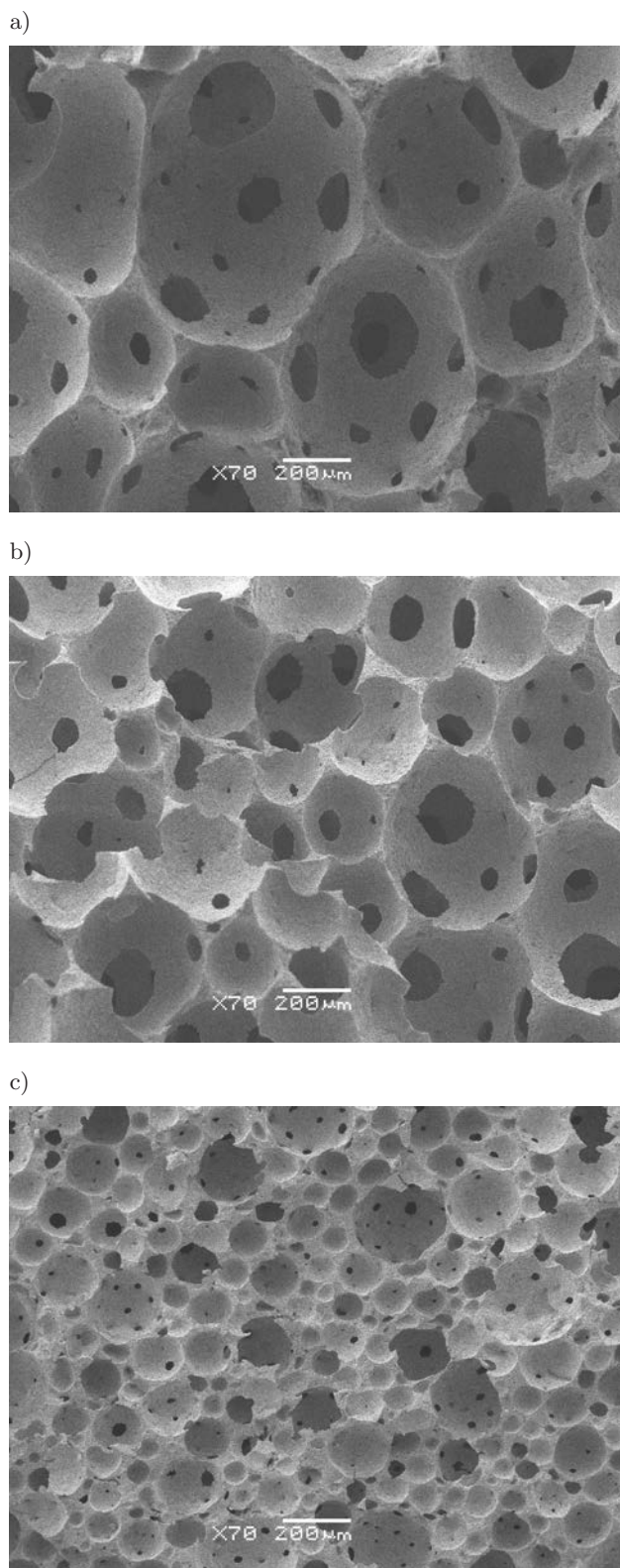
Fig. 1. SEM cross-section of alumina foams having porosity of: a) 90%, b) 88%, and c) 72%.
