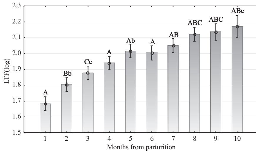
Fig. 1 Mean and \pm SD of milk lactoferrin concentration (log transformed) during lactations; A,B,C The same letter indicate high significant ( P < 0.01 ) differences in the means; a,b,c The same letter indicate significant ( P < 0.05 ) differences in the means.
