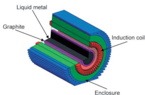
Fig. 1. Scheme of an electromagnetic stirrer applied in the studies
