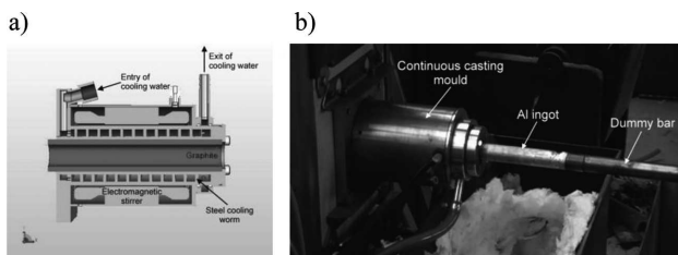
Fig. 8. Scheme (a) and view (b) of continuous casting mould containing electromagnetic stirrer, which is a part of stand of continuous casting of Al and its alloys, developed and manufactured at Foundry Department of Silesian University of Technology in Gliwice, Poland
