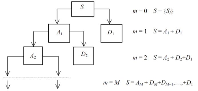
Fig. 1. Block diagram of signal S[n] representation as the sum of approximation and details [5].
