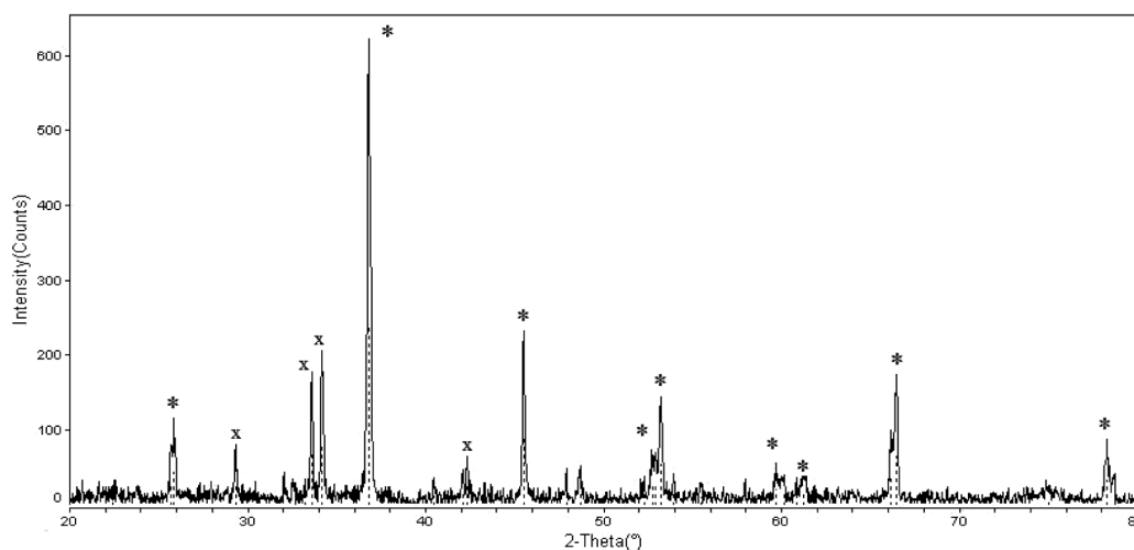
Fig. 3. XRD diagram of barium titanate ceramics sintered at 1200°C for 6h., * denotes tetragonal and x unknown phase
