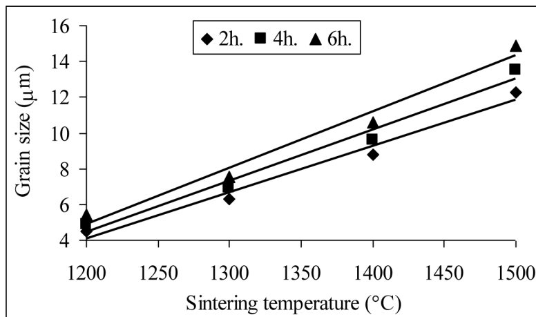
Fig. 4. Grain size vs. sintering temperature graphs for BTLP-1
