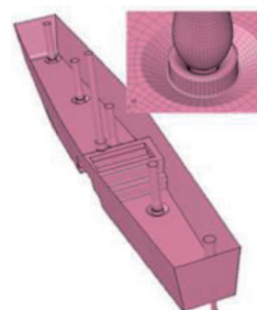
Fig. 2. The tundish geometry of CCM No.1 with the surface at 0.6 m level– variant for 20 tons of steel in the tundish
