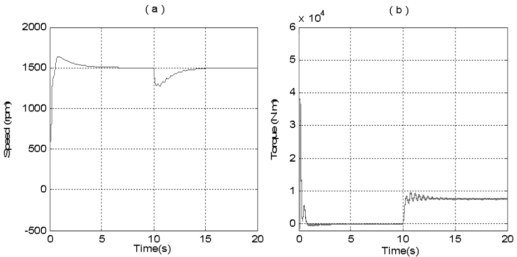
Figure 13. Induction motor mechanical features.
