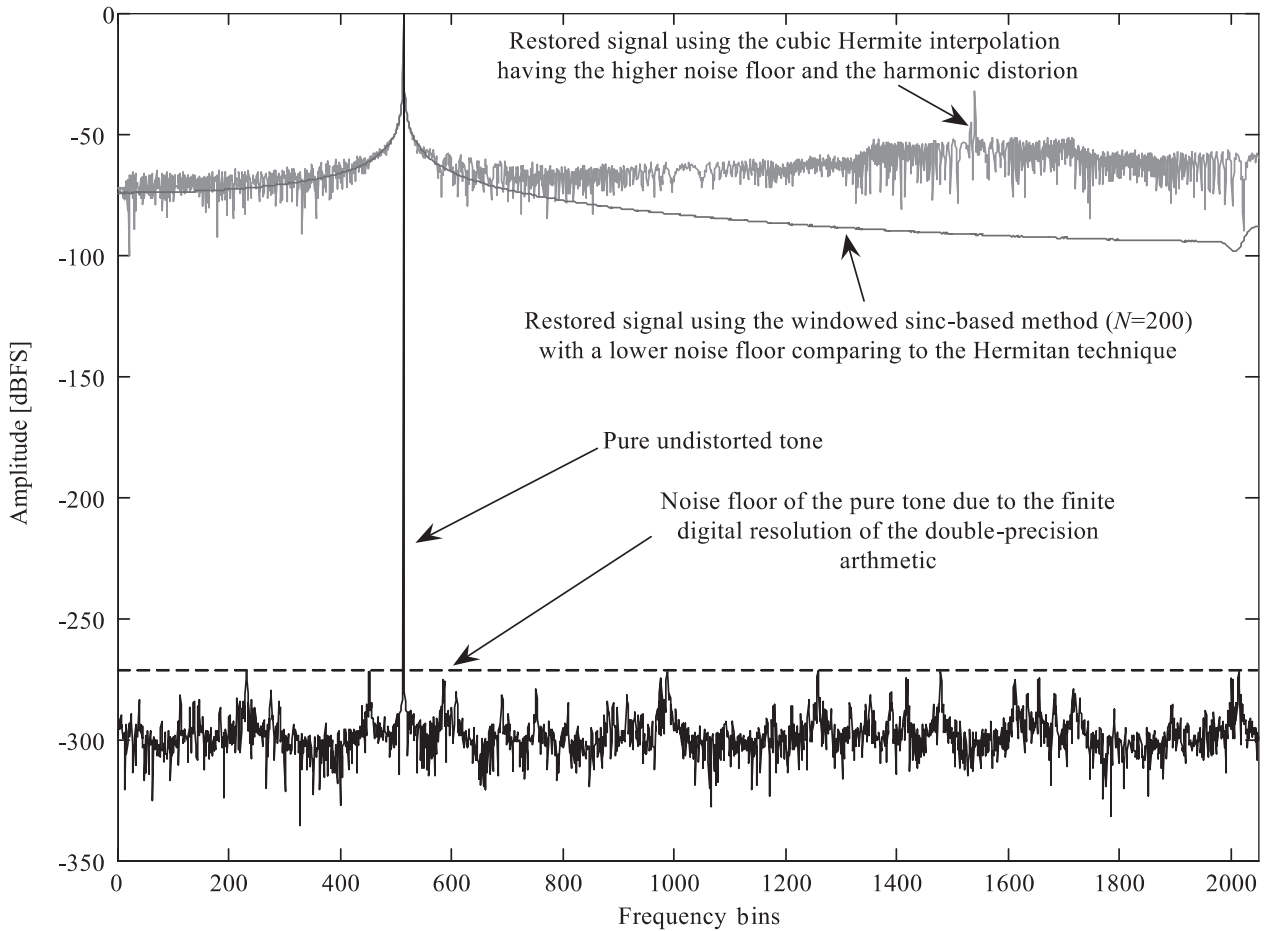
Fig. 8. Amplitude spectra of two signals restored by the windowed sinc-based method with the von Hann window and the polynomial-based cubic Hermite method, and the spectrum of a tone undistorted by wow
