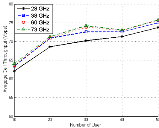
Fig. 3. Number of User vs Average Cell Throughput
