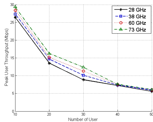
Fig. 4. Number of User vs Peak User Cell Throughput
