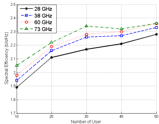
Fig. 5. Number of User vs Spectral Efficiency
