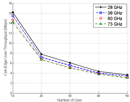
Fig. 2. Number of User vs Cell-Edge User Throughput
