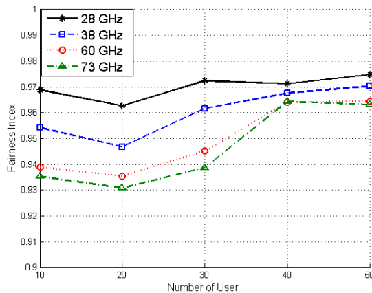
Fig. 6. Number of User vs Fairness Index
