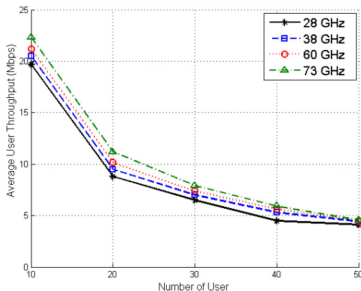
Fig. 1. Number of User vs Average User Throughput
