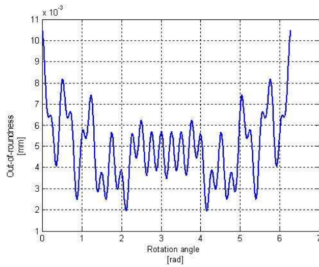
Fig. 7. The roundness profile given by formula (10).
