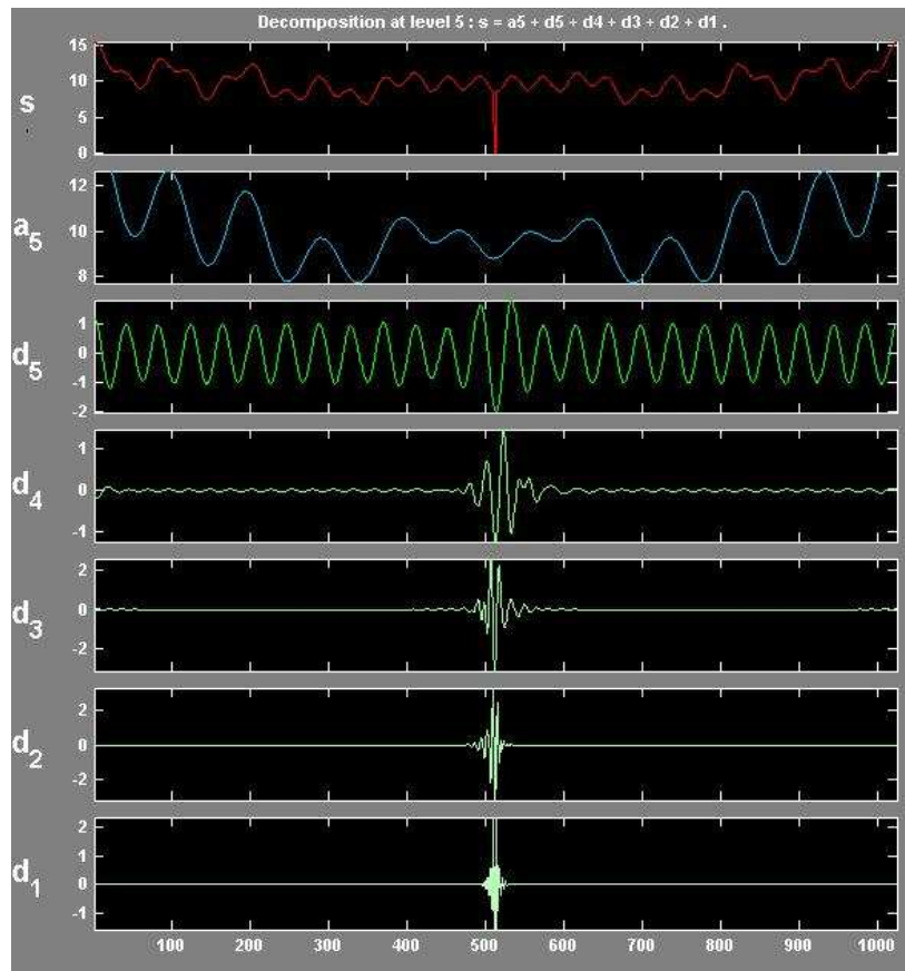
Fig. 11. Wavelet decomposition of the profile shown in Fig. 9 (type of mother wavelet – discrete Meyer wavelet, number of decomposition levels – 5).
