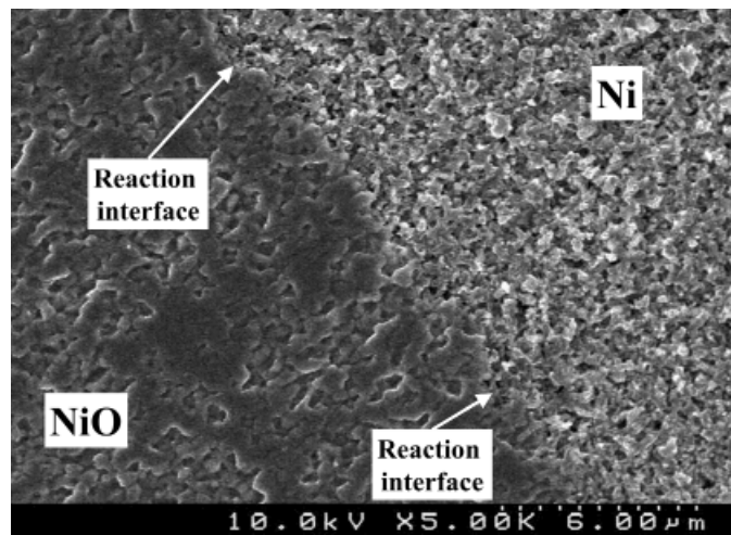
Fig. 6. Image of a partially reduced Goro oxide particle at 623 K (350°C)
