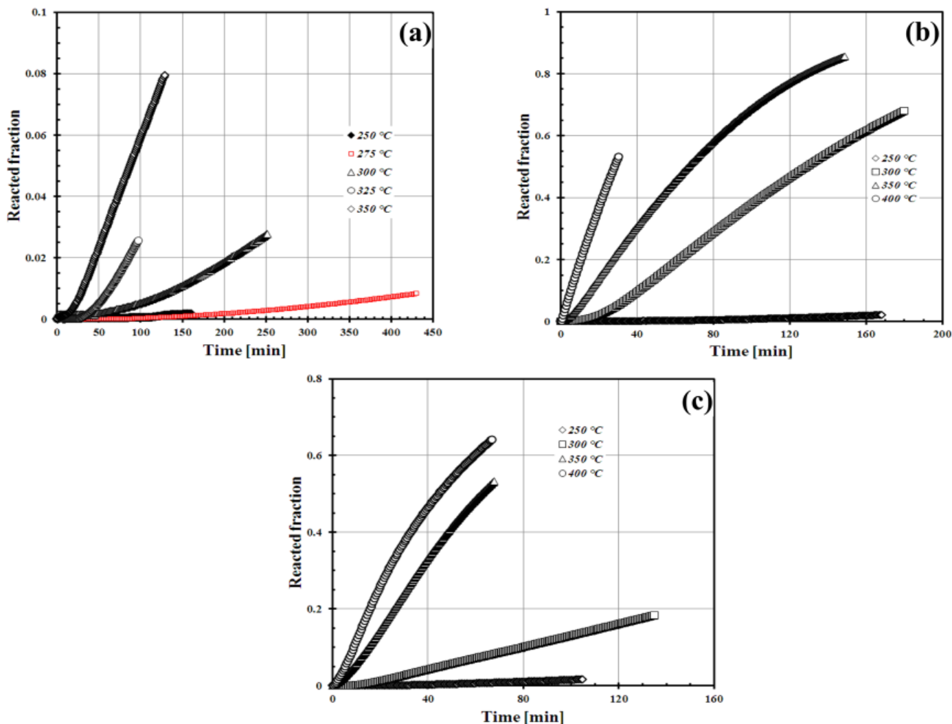
Fig. 3. Reacted fraction during the reduction between 523 and 673 K (250 and 400°C) in a gas containing 35%vol H 2 of (a) Goro oxide, (b) Tokyo oxide and (c) Sinter 75 oxide
